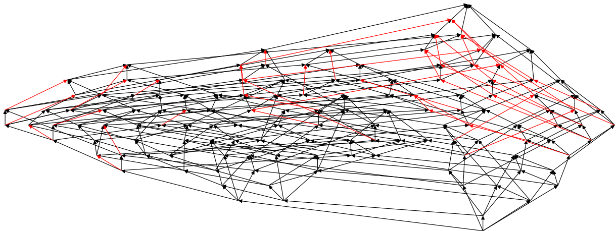
FIGURE 7. Hasse diagram of \mathcal{S}_6 = (\mathcal{D}_6, \leq) (black edges). The Tamari lattice \mathcal{T}_6 = (\mathcal{D}_6, \preceq) can be viewed by considering black and red edges.
